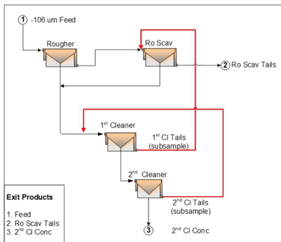
Figure 1: LCT-3 Flowsheet
